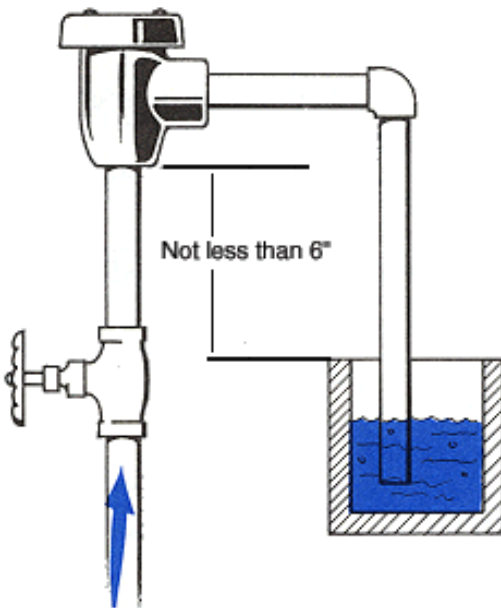
Atmospheric Vacuum Breaker Typical Installation
